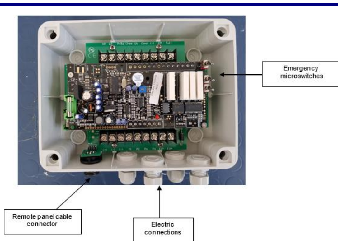
COMPUTER BOX WITH SWITCHES FIG. 3-10
