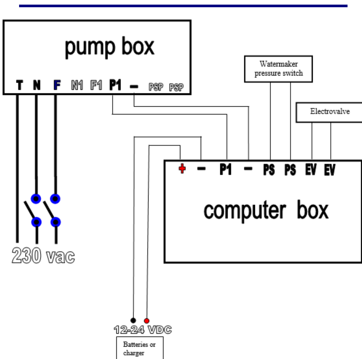
WIRING LOGIC SCHEME 230 VAC FIG. 4-4
