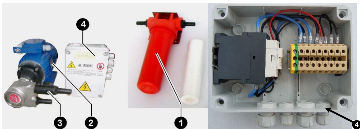
PUMP GROUP AND FILTER 230 V AC FIG. 3-6
